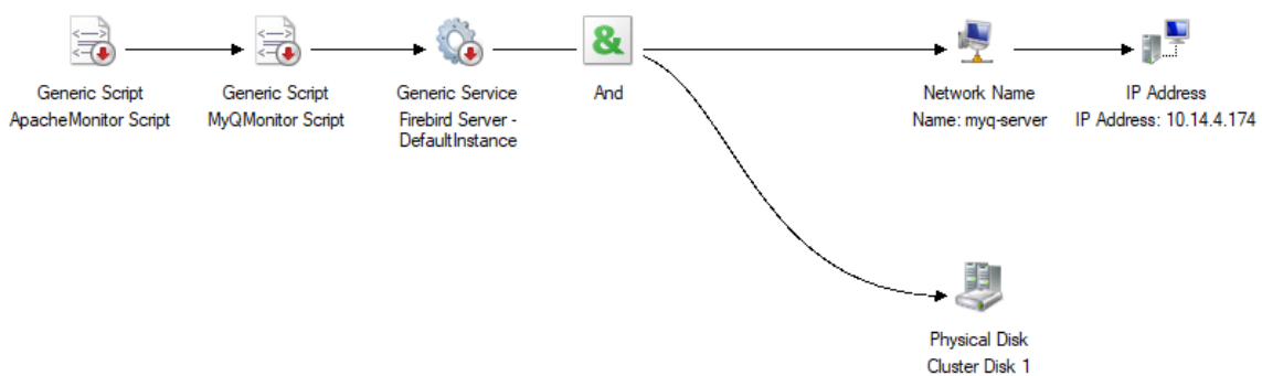
8 Dependency graph of the cluster on the MyQ server
