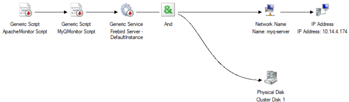
1 Dependency graph of the cluster on the MyQ server
