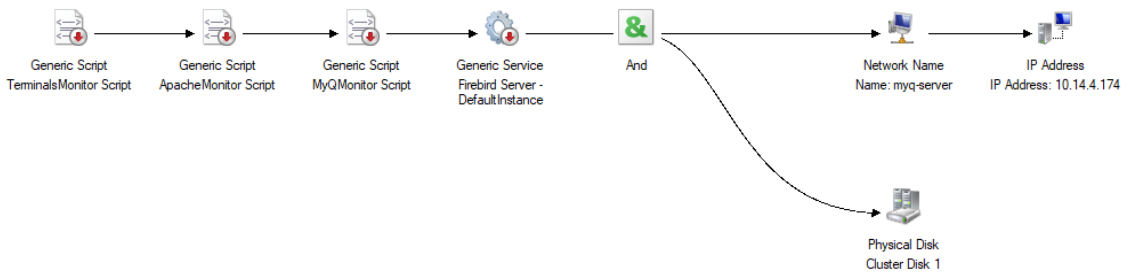
2 Dependency graph of the cluster with embedded terminal on the MyQ server
